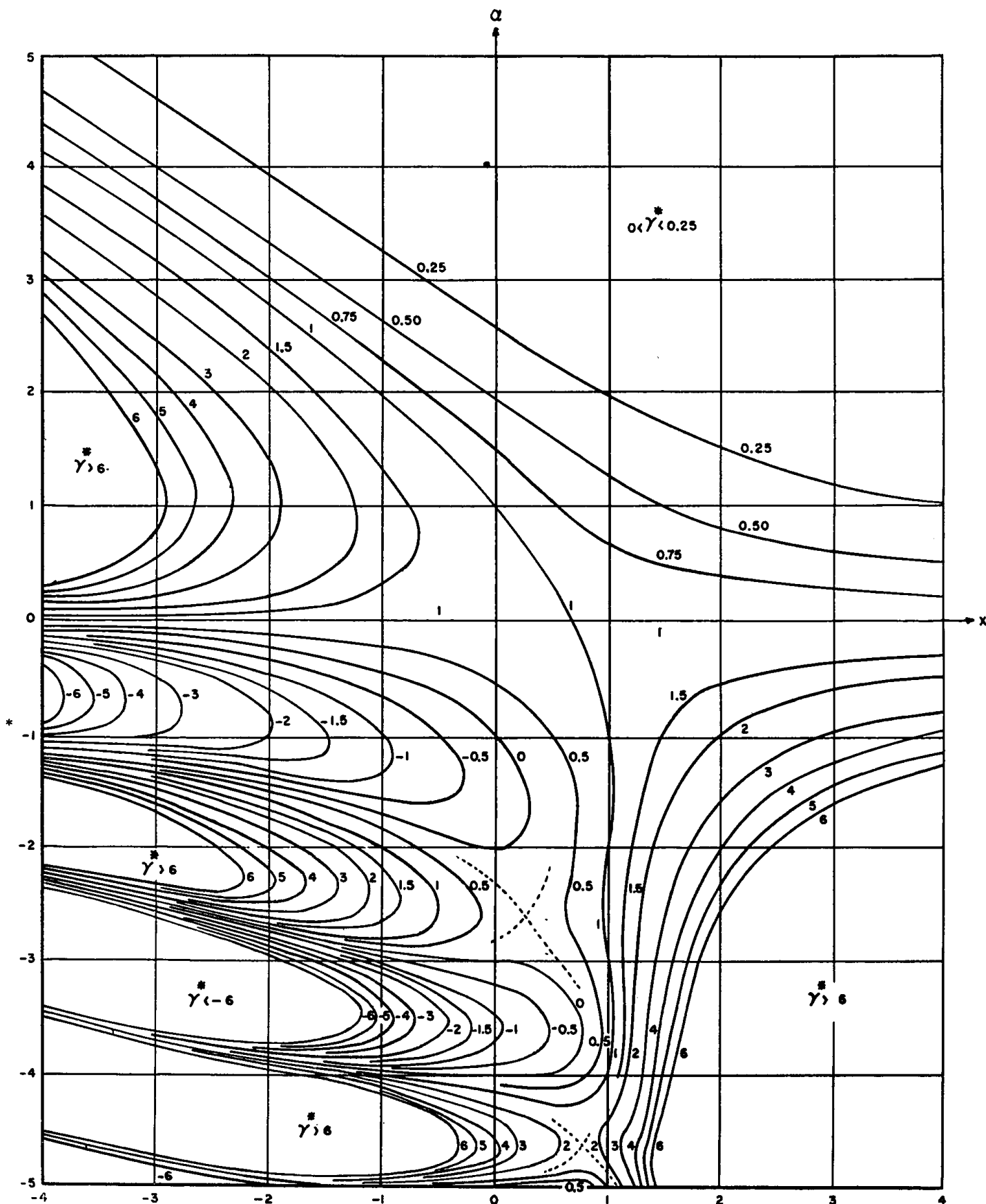
FIGURE 6.3. Incomplete gamma function.
