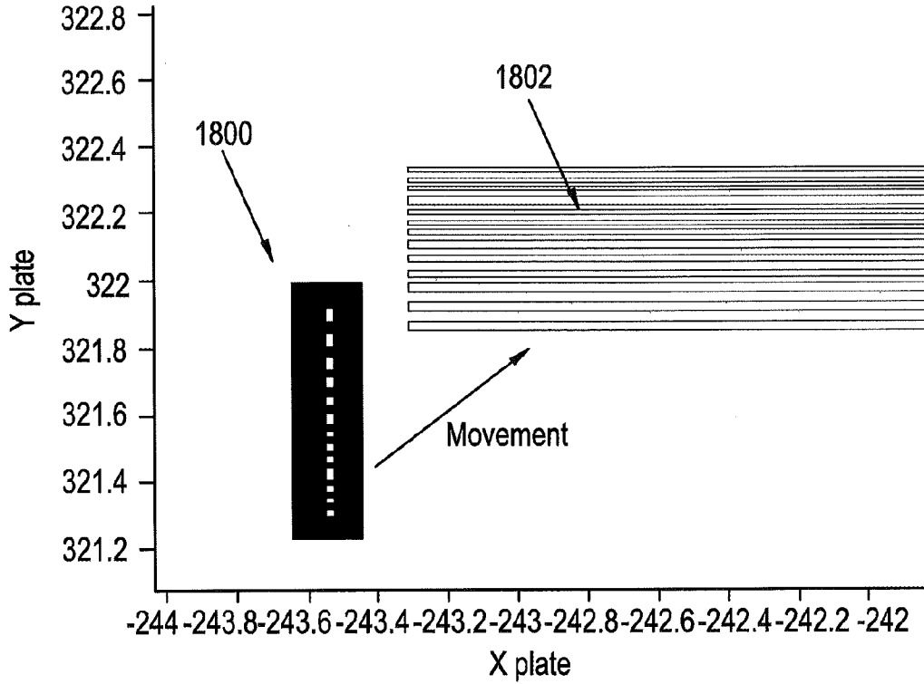
Calibration pattern in calibration plate coordinate system
